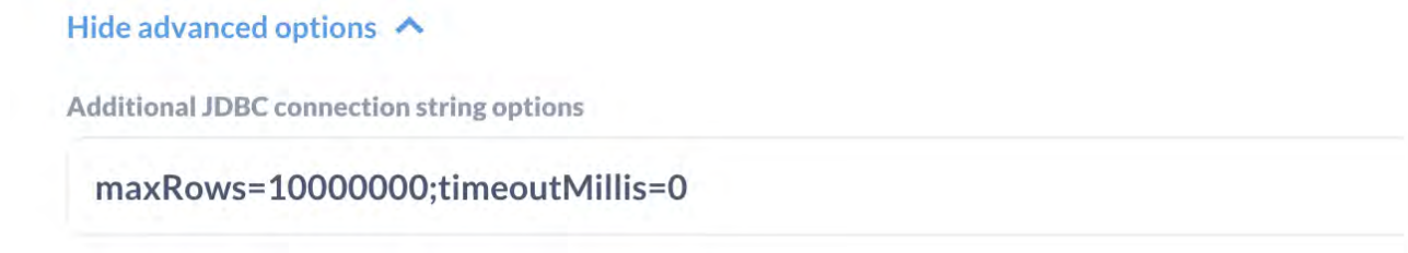
Figure 8: Additional JDBC connection string options sets the maxRows and timeoutMillis parameters.
