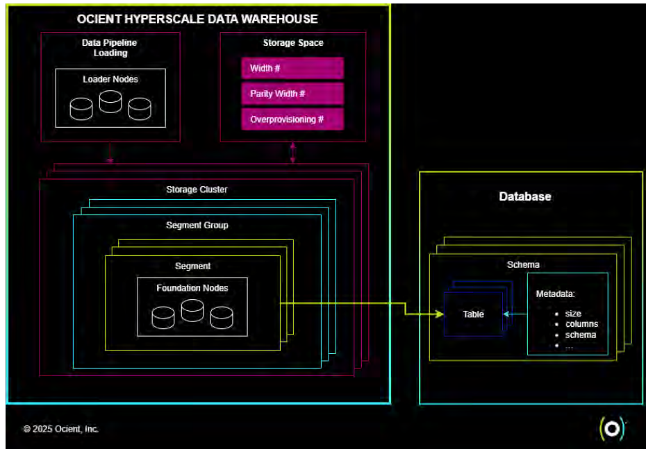
Figure 22: Ocient Hyperscale Data Warehouse contains Foundation Nodes in segments grouped into segment groups that are grouped into storage clusters. Tables in schemas with metadata are stored in segments.
