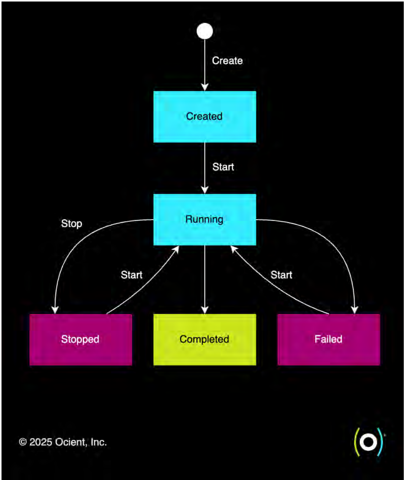
Figure 10: Pipeline status state machine with created, running, stopped, completed, and failed states
