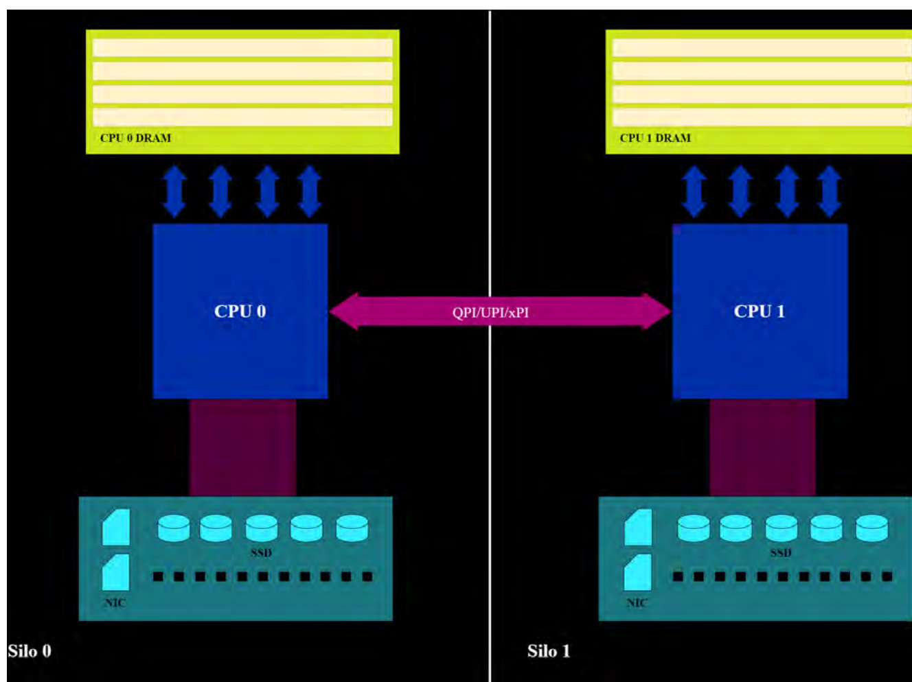
Figure 28: Multiple NUMA-aware processing silos per node
