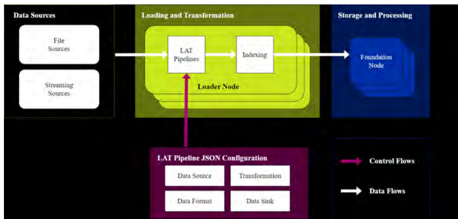
Figure 33: LAT pipeline JSON configuration with data flow from data sources to storage and processing
