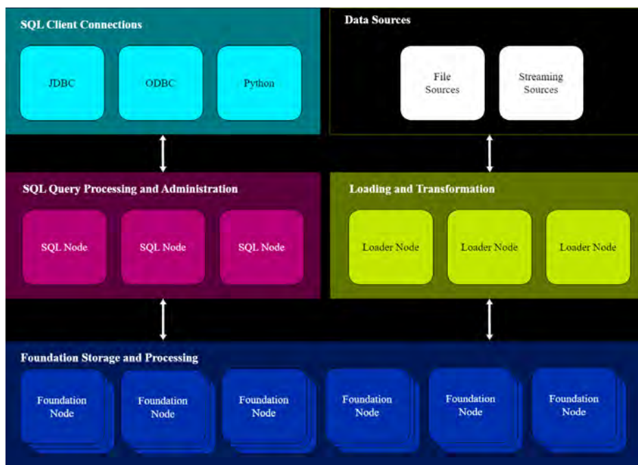
Figure 11: Ocint loading architecture that consists of SQL client connections that interface with SQL Nodes, data sources that interface with Loader Nodes, and SQL and Loader Nodes interface with Foundation Nodes for storage and processing.
