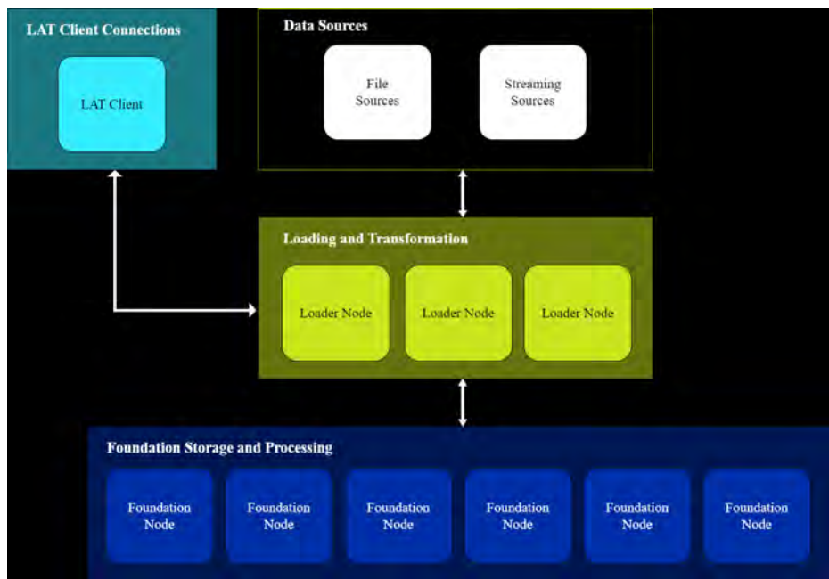
Figure 32: Loading and transformation into foundation storage
