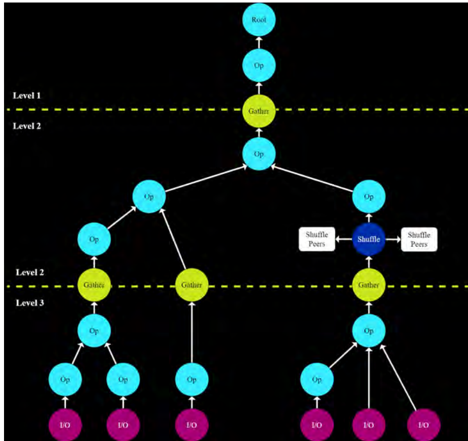
Figure 30: Query tree operators for three levels
