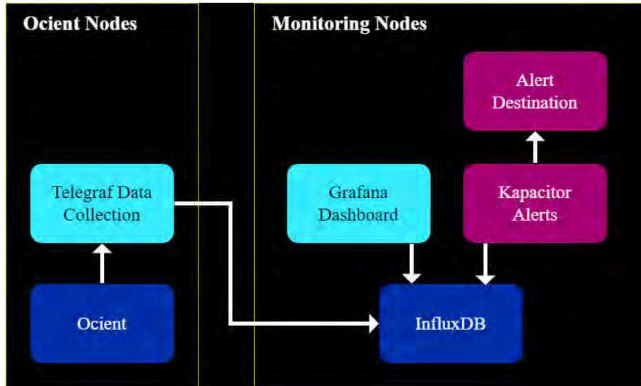
Figure 15: Monitoring example with Telegraf data collection into InfluxDB with Grafana dashboard and Kapacitor alerts
