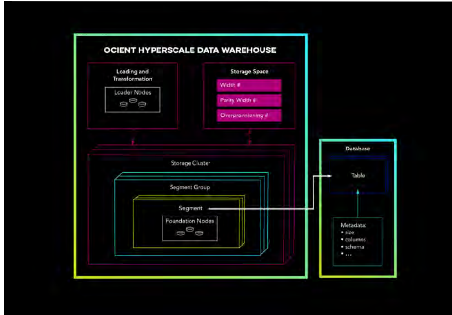
Figure 14: Ocient Hyperscale Data Warehouse contains Foundation Nodes in segments grouped into segment groups that are grouped into storage clusters. Tables with metadata are stored in segments
