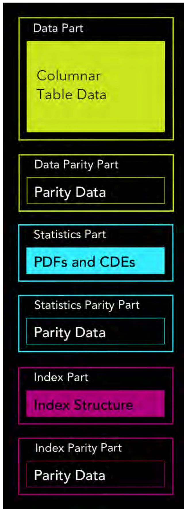
Figure 23: Example segment and segment part structure that contains data, statistics, and index parts and corresponding parity data
