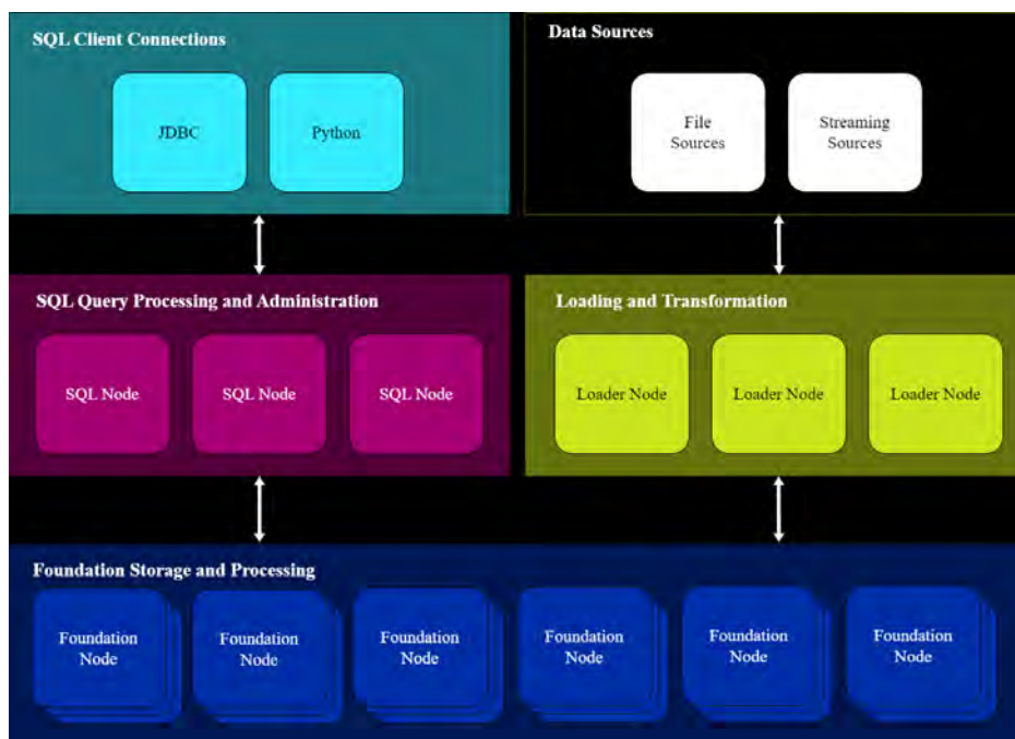
Figure 21: Ocient architecture diagram that shows the relationship between data sources, loading and transformation of the data, and data storage
