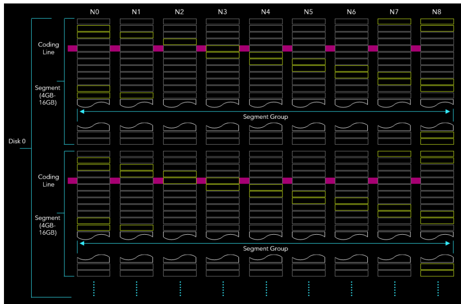
Figure 24: Erasure coding example where N = 7 and K = 2
