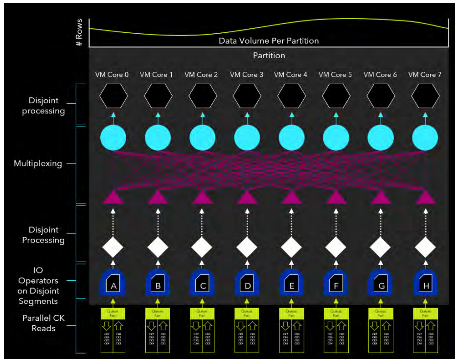
Figure 27: Parallel VM core operation with balanced data flow
