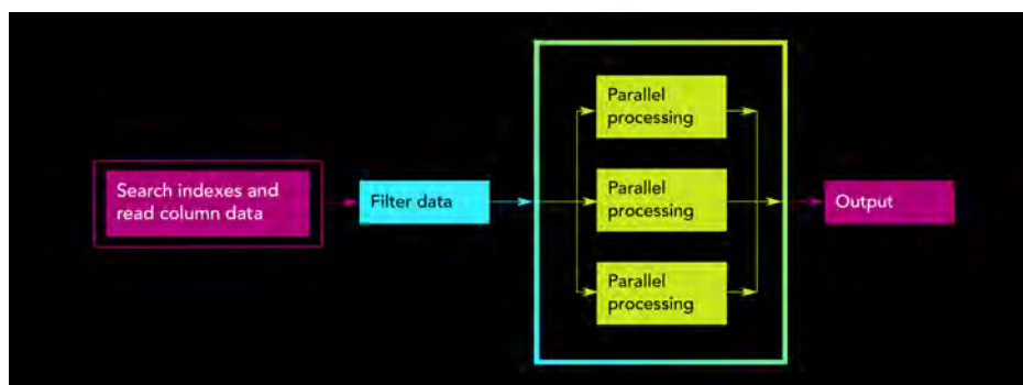
Figure 26: Simple I/O pipeline example that contains a pipeline and its elements
