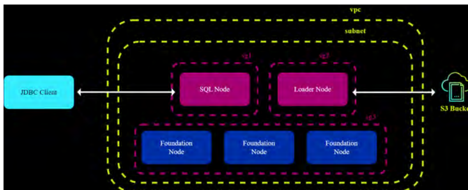
Figure 13: Virtual private cloud for loading data from an S3 bucket using a JDBC client
