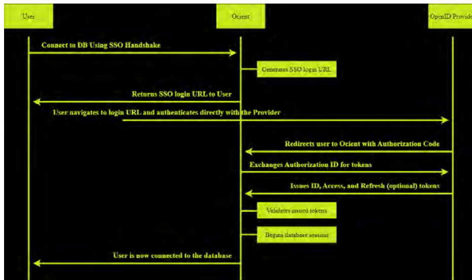
Figure 12: Sequence of authentication flow
