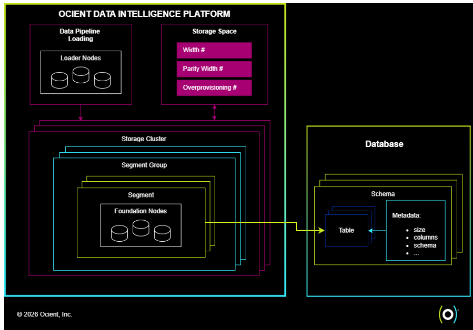
Figure 22: Ocient Data Intelligence Platform contains Foundation Nodes in segments grouped into segment groups that are grouped into storage clusters. Tables in schemas with metadata are stored in segments.
