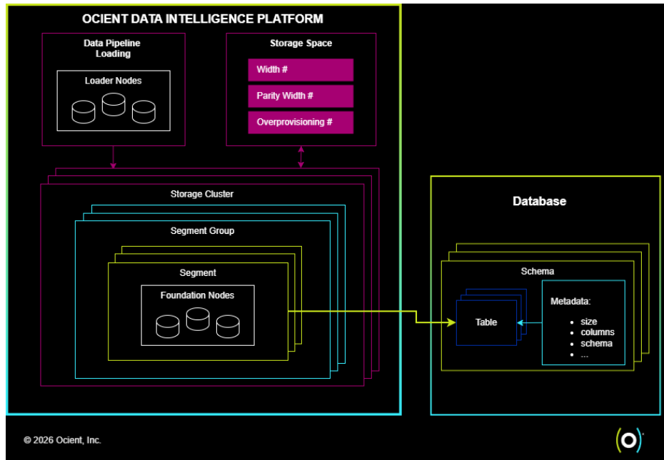
Figure 14: Ocient Data Intelligence Platform contains Foundation Nodes in segments grouped into segment groups that are grouped into storage clusters. Tables in schemas with metadata are stored in segments.
